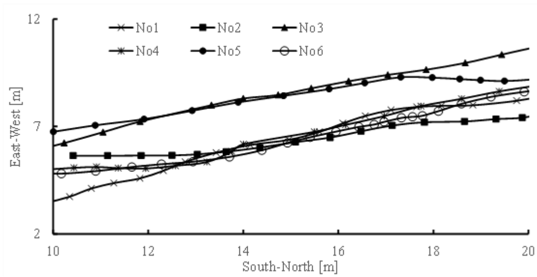
Appendix Figure 3. Position information from the SA-GNSS receiver in the apple field.
