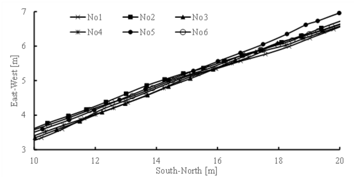
Appendix Figure 1. Position information from the RTK-GNSS receiver in the apple field.
