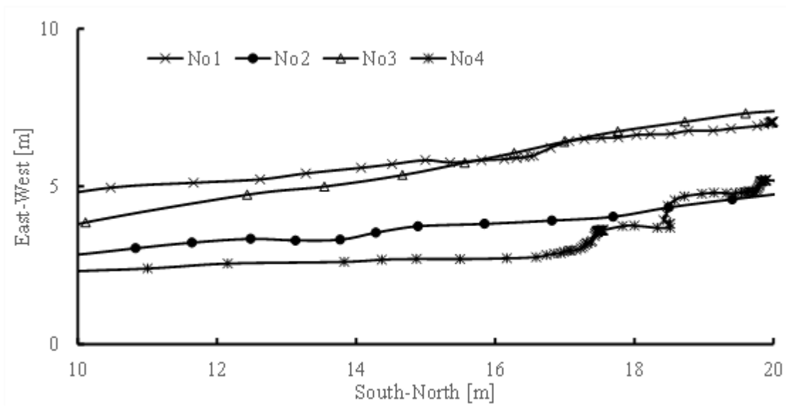
Appendix Figure 4. Position information from the SA-GNSS receiver in the pear field.
