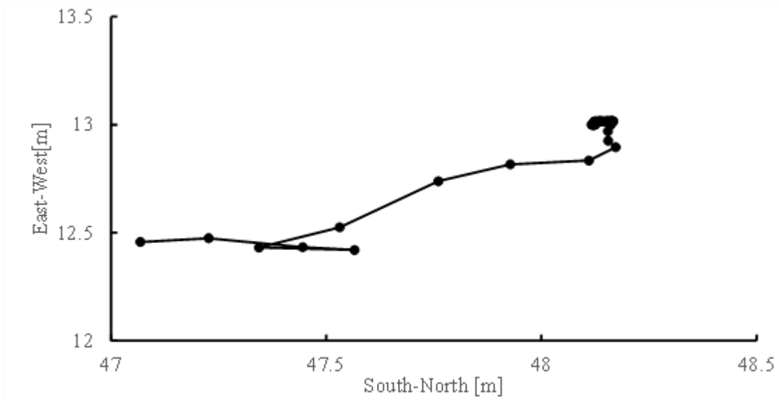
Appendix Figure 5. Positioning plots for the SA-GNSS during a halt at the midpoint.
