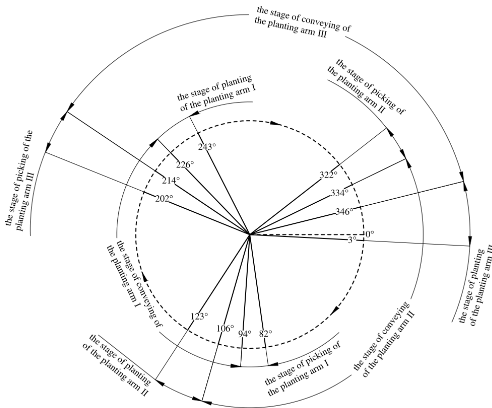
Appendix Figure 5. Work cycle diagram.
