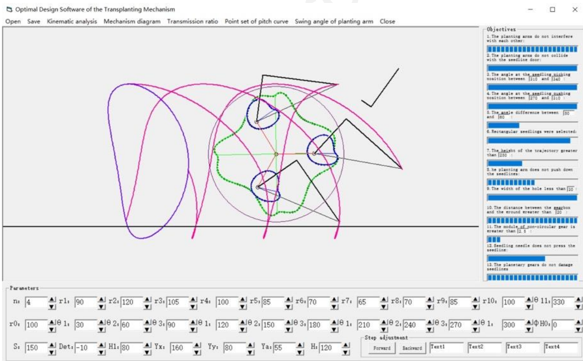
Appendix Figure 2. Optimal design software of the transplanting mechanism.
