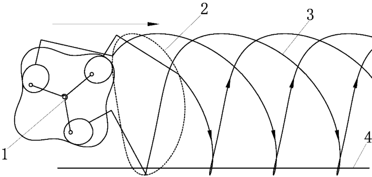
Appendix Figure 1. Trajectory of the transplanting mechanism. 1. Transplanting mechanism with differential internal engagement non-circular planetary gear trains; 2. Relative motion trajectory; 3. Absolute motion trajectory; 4. Ground.
