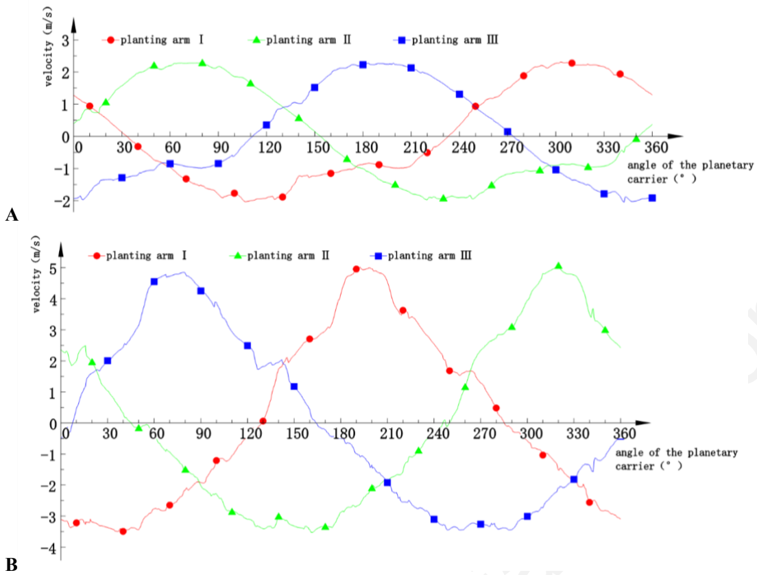
Appendix Figure 4. Velocities of the planting arms. A) Velocity in the X direction; B) Velocity in the Y direction.
