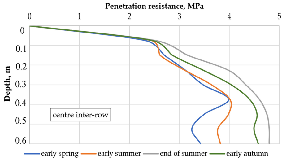
Figure 7. Penetration resistance curves recorded in the centre inter-row for four periods during the growing season in Bosco vineyard.
