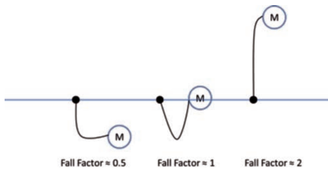
Figure 1. Fall factor definition.
